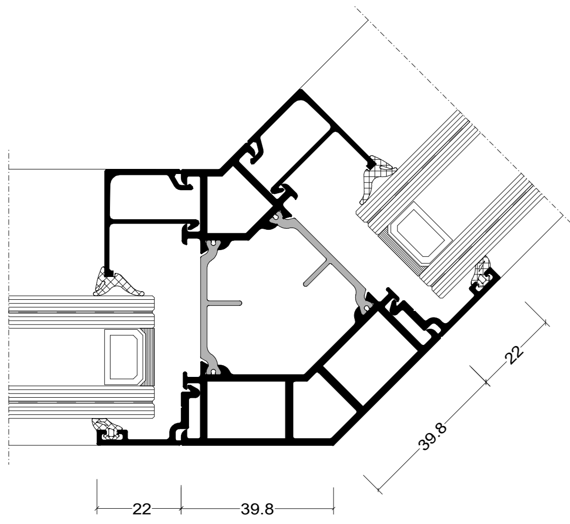
45 graden hoekoplossing
