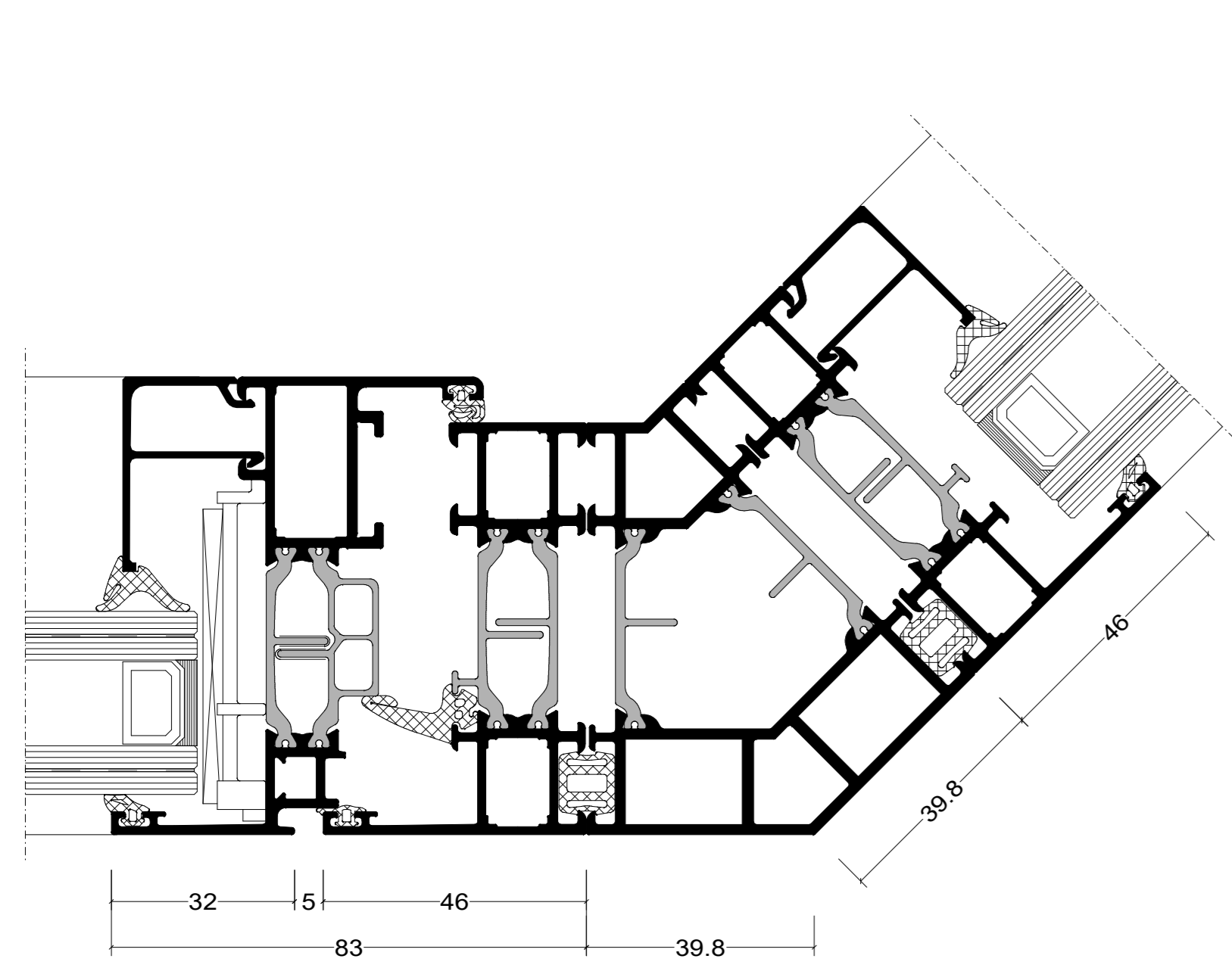
45 graden koppeling
