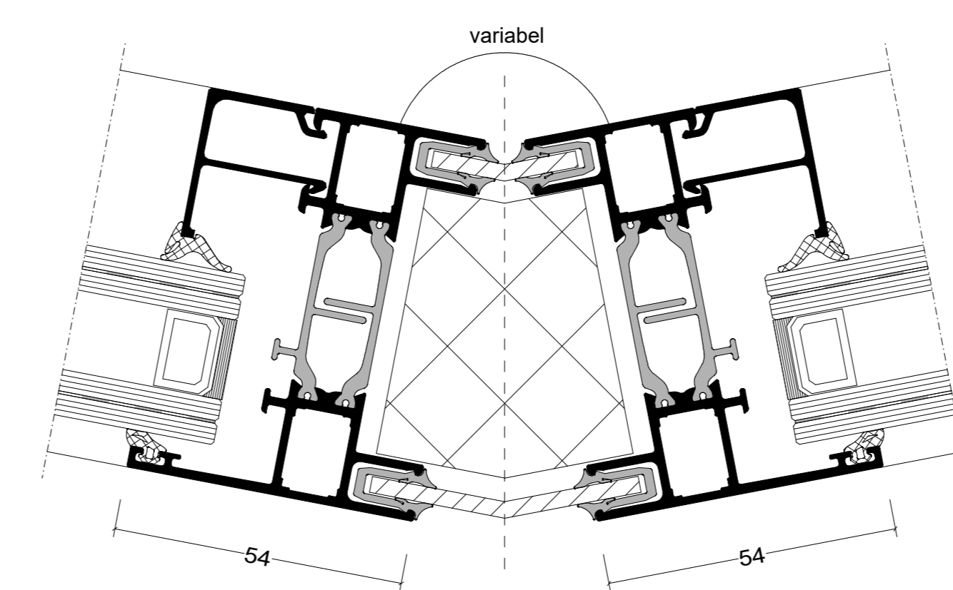
Variabele hoekoplossing
