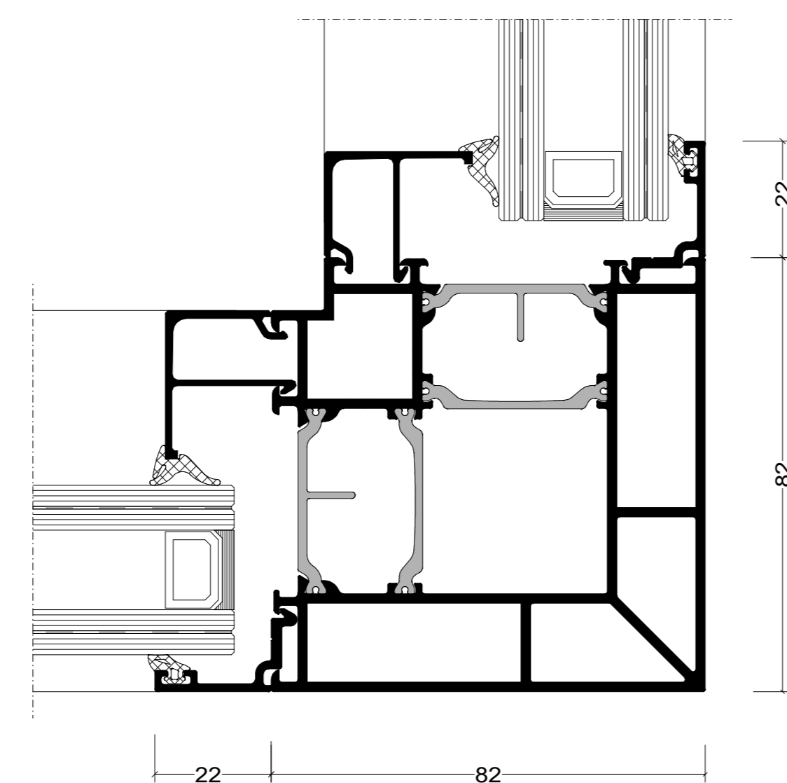
90 graden hoekoplossing
