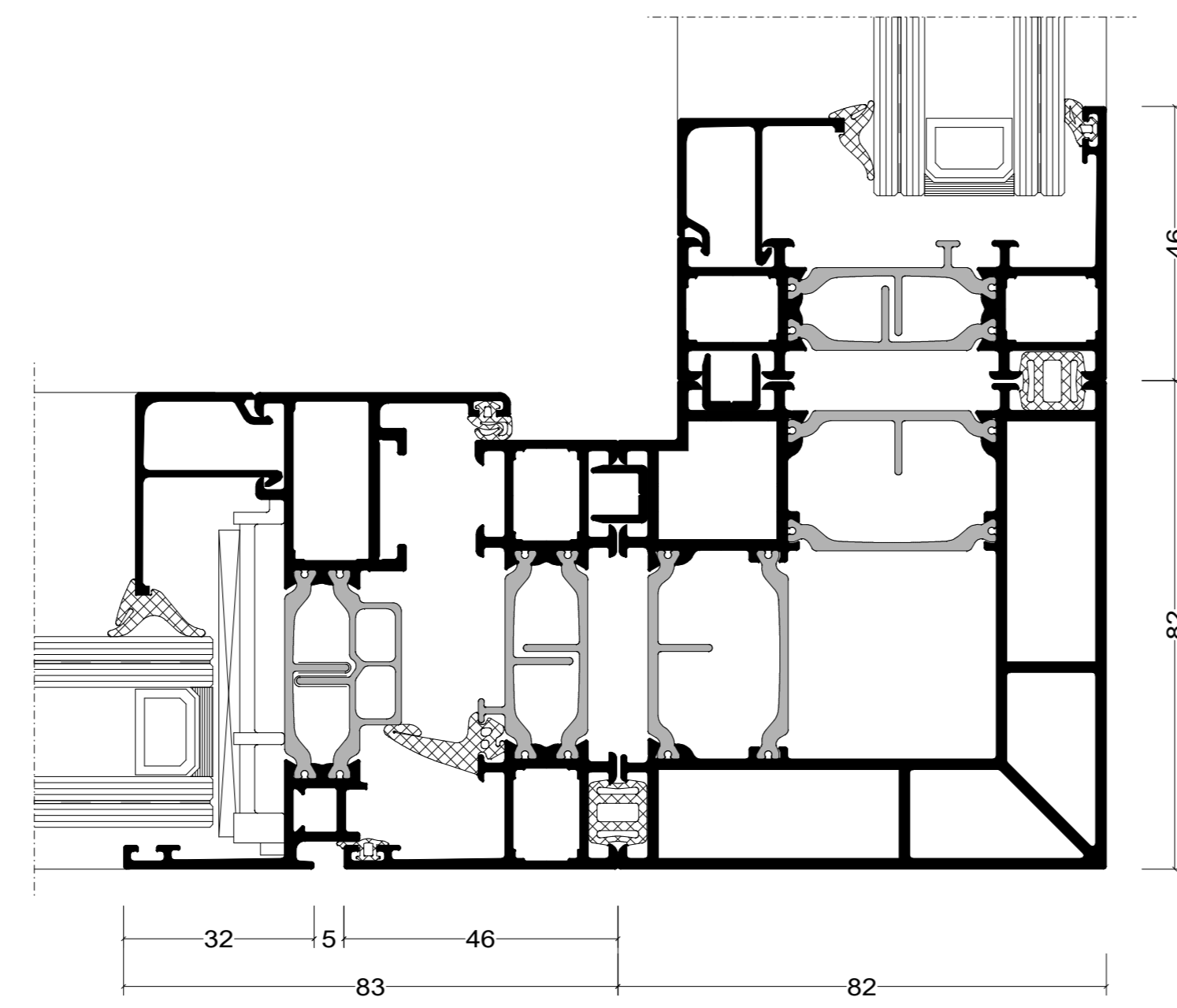
90 graden koppeling
